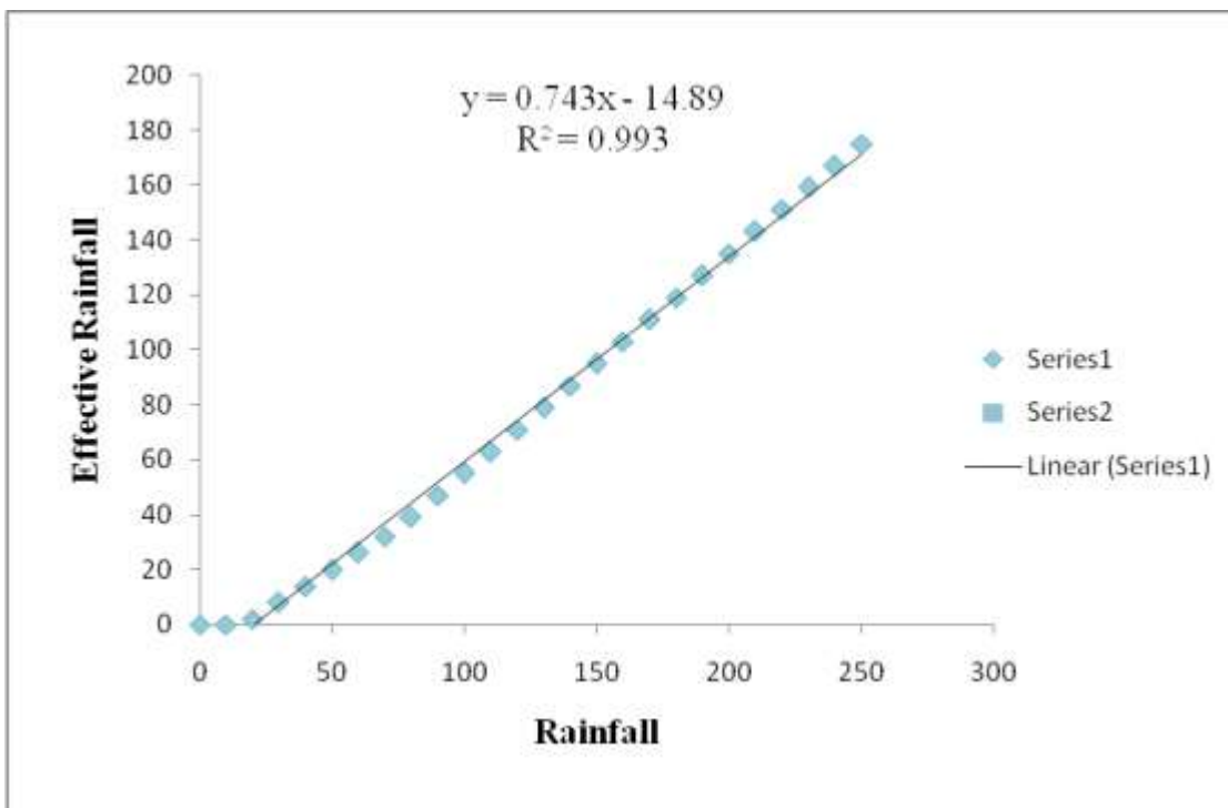
Fig. 2 Relation between rainfall and effective rainfall.
