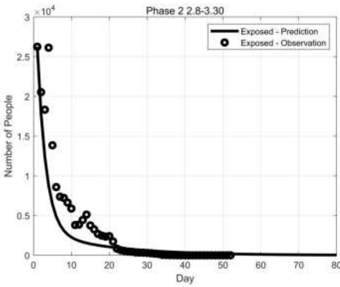
Fig.6: Result of curve fitting for the exposed E(t) in Phase 2 (2020.2.8 - 2020.3.30)
