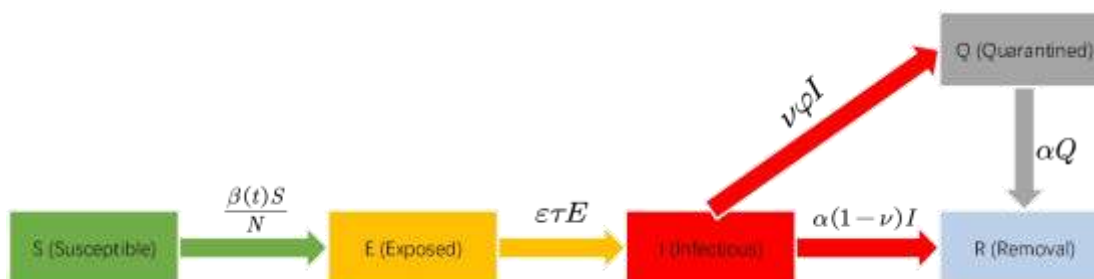
Fig.2: 2020.2.8 - 2020.3.30, SEIQR model, where ( ) ( ) ( )
