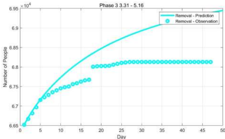
Fig.11: Result of curve fitting for the removal R(t) in Phase 3 (2020.3.31-2020.5.16)
