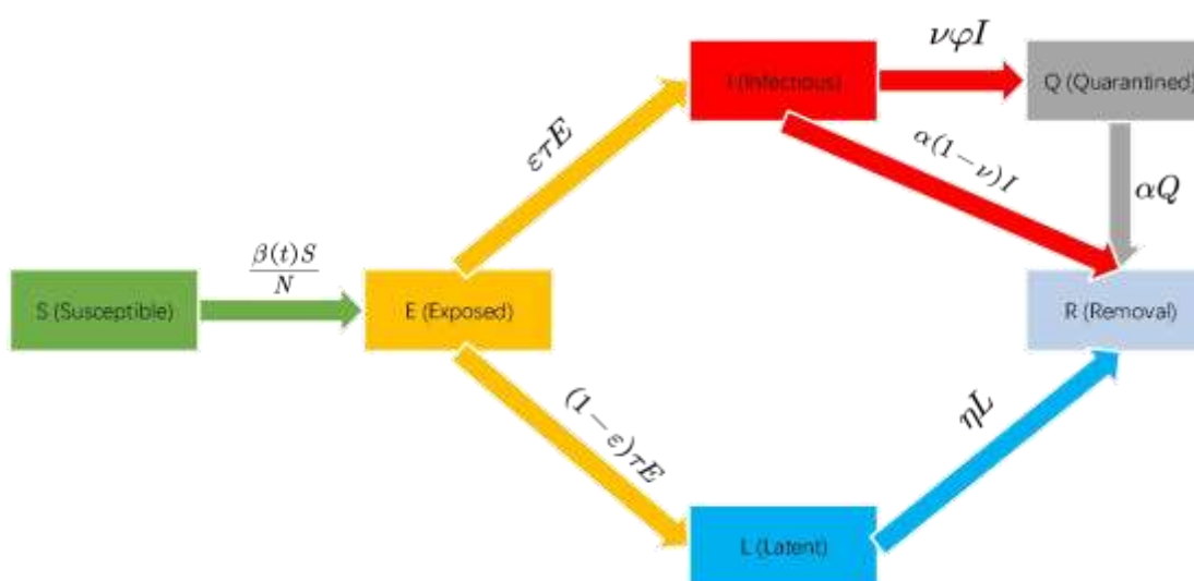
Fig.3: 2020.3.31 - 2020.5.16, SEIQLR model, where ( ) ( ) ( ) ( )
