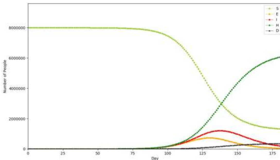
Fig.5: Result of SEIR simulation
