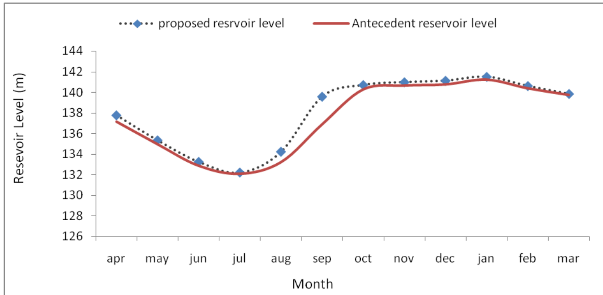
Fig. 4: reservoir level rule curve for Kainji Dam
