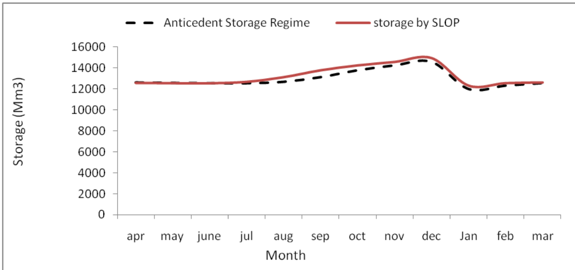
Fig. 3: Kainji reservoir storage rule curve
