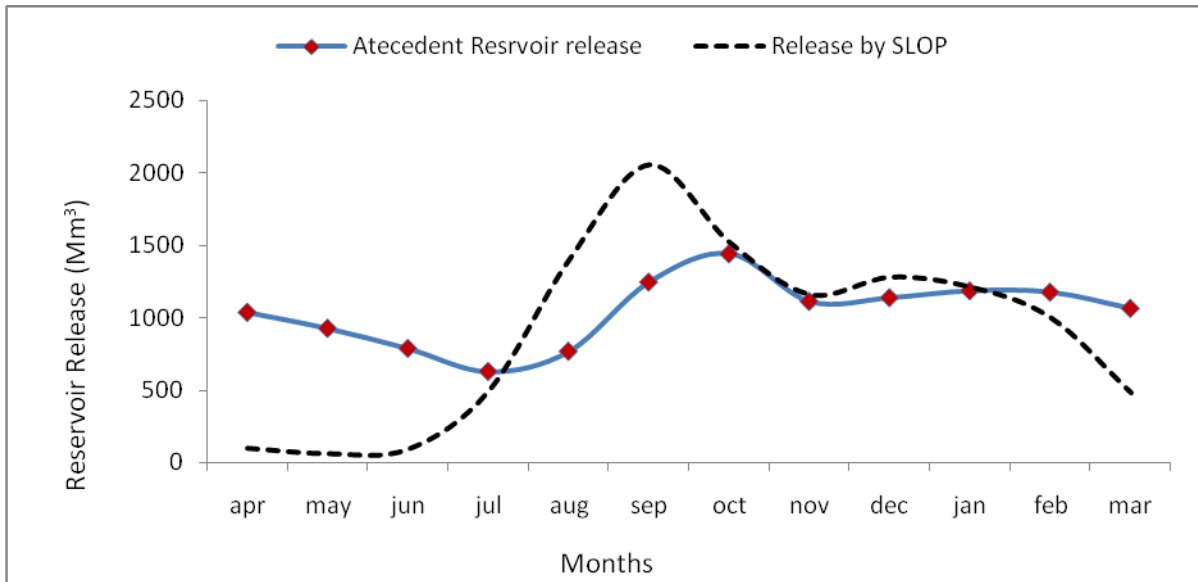
Fig. 5: Reservoir release rule curve for Kainji Dam
